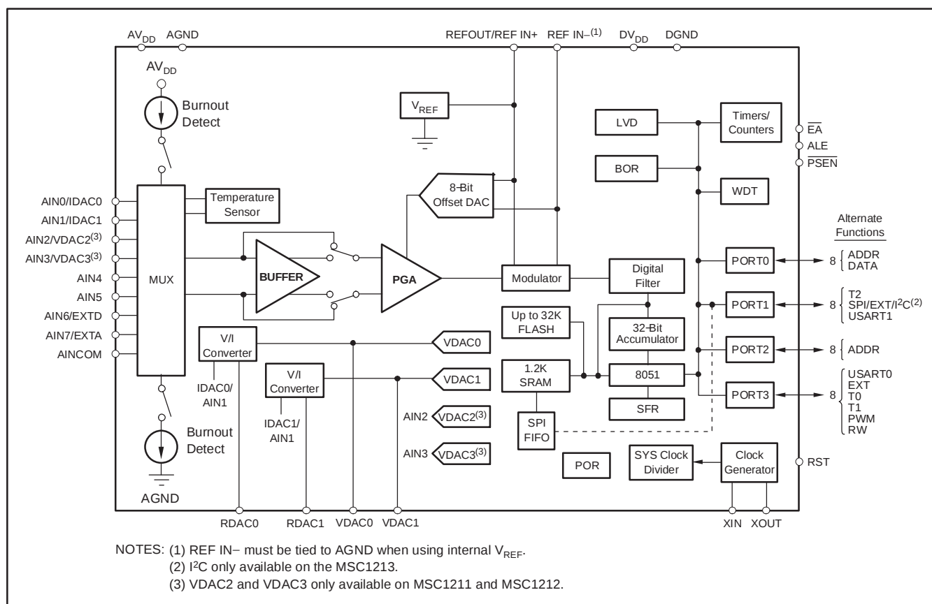
Figure 8. Block Diagram
