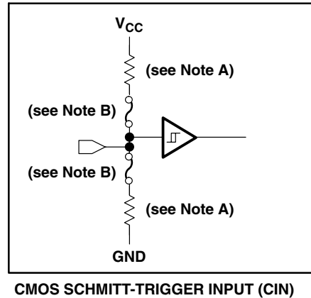
CMOS SCHMITT-TRIGGER INPUT (CIN)
