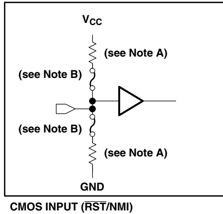
CMOS INPUT ( \overline{\text{RST}}/\text{NMI} )
