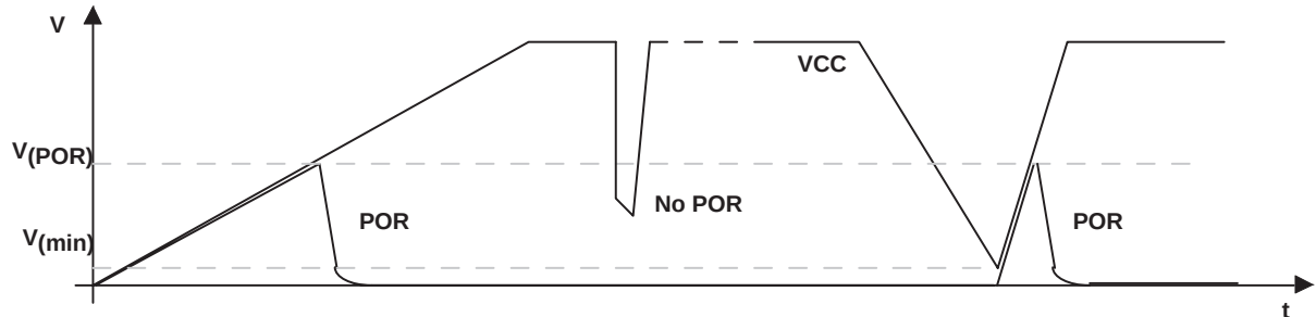
Figure 3. Power-On Reset (POR) vs Supply Voltage
