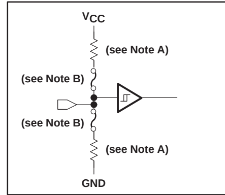
CMOS SCHMITT-TRIGGER INPUT ( \text{CIN} )
