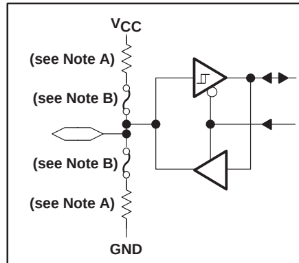
I/O WITH SCHMITT-TRIGGER INPUT ( \text{P0.x} , \text{TP5} )
