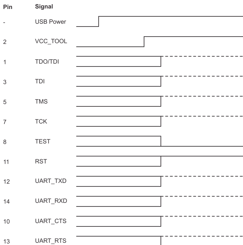
Figure B-85. Pin States After Power-Up
