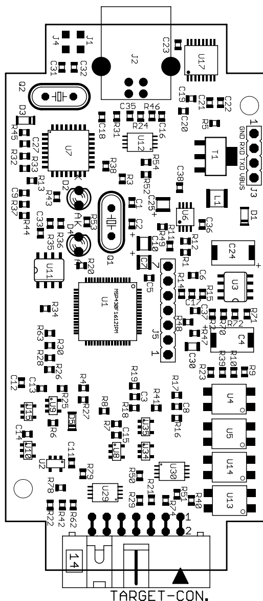
Figure B-92. MSP-FET430UIF USB Interface, PCB
