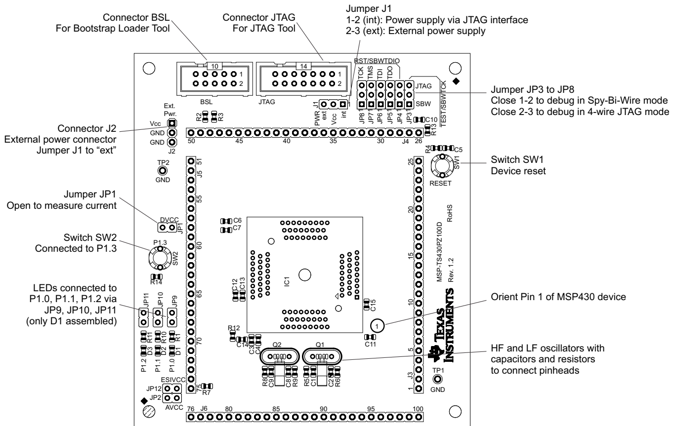
Figure B-62. MSP-TS430PZ100D Target Socket Module, PCB
