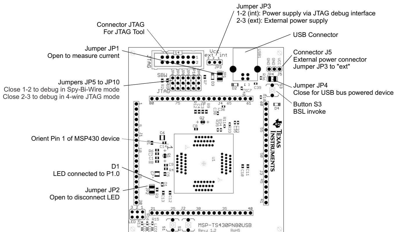
Figure B-52. MSP-TS430PN80USB Target Socket Module, PCB
