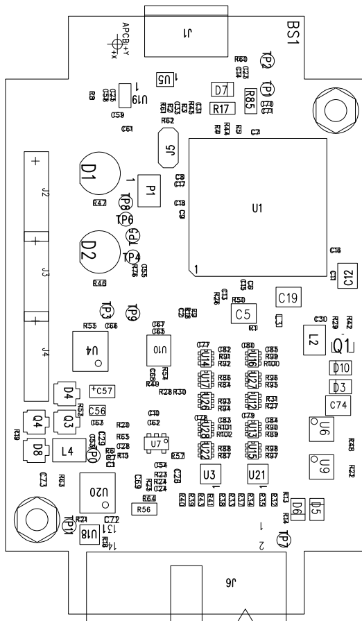
Figure B-82. MSP-FET USB Debugger, PCB (Top)
