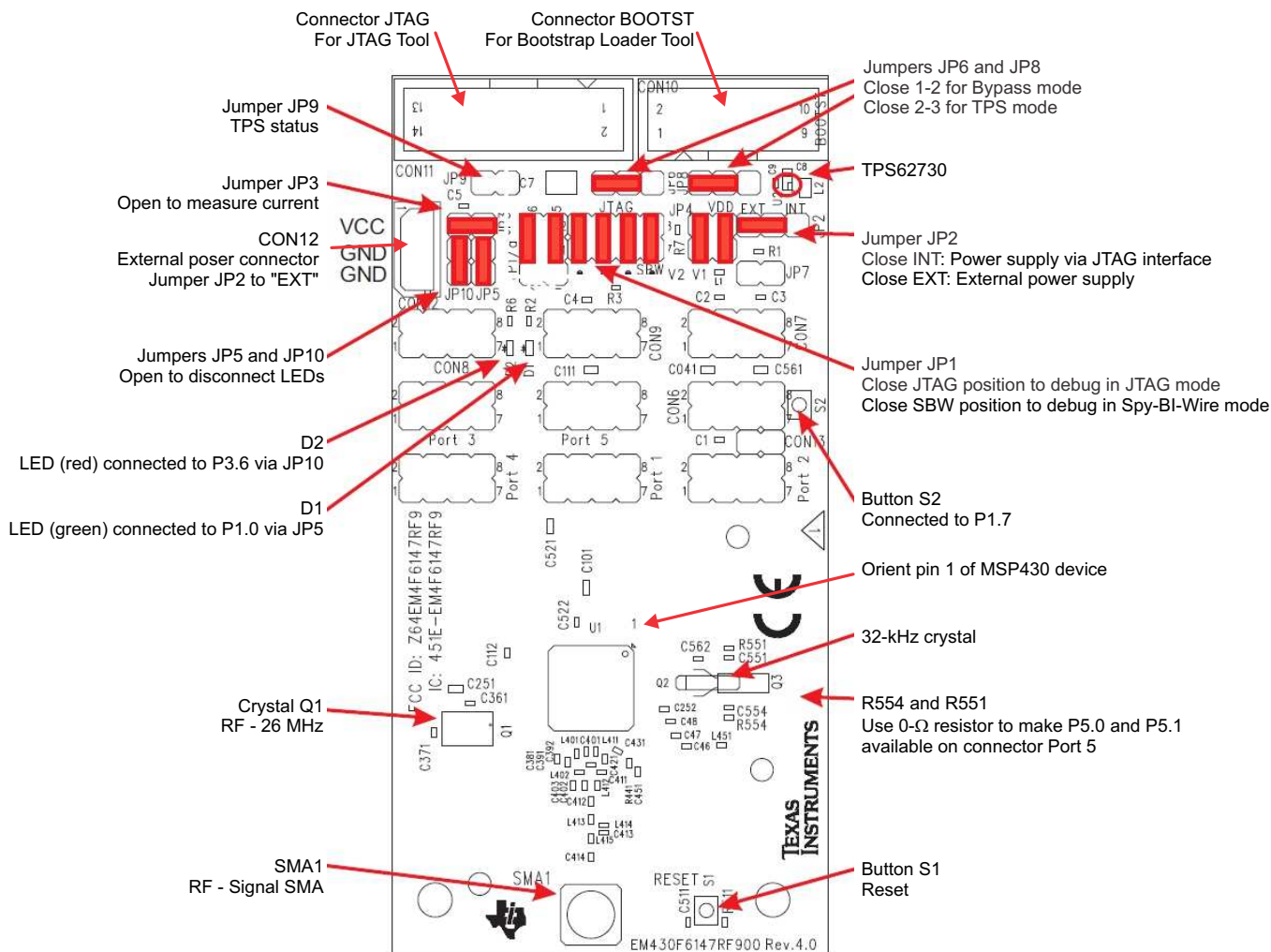
Figure B-74. EM430F6147RF900 Target Board, PCB
