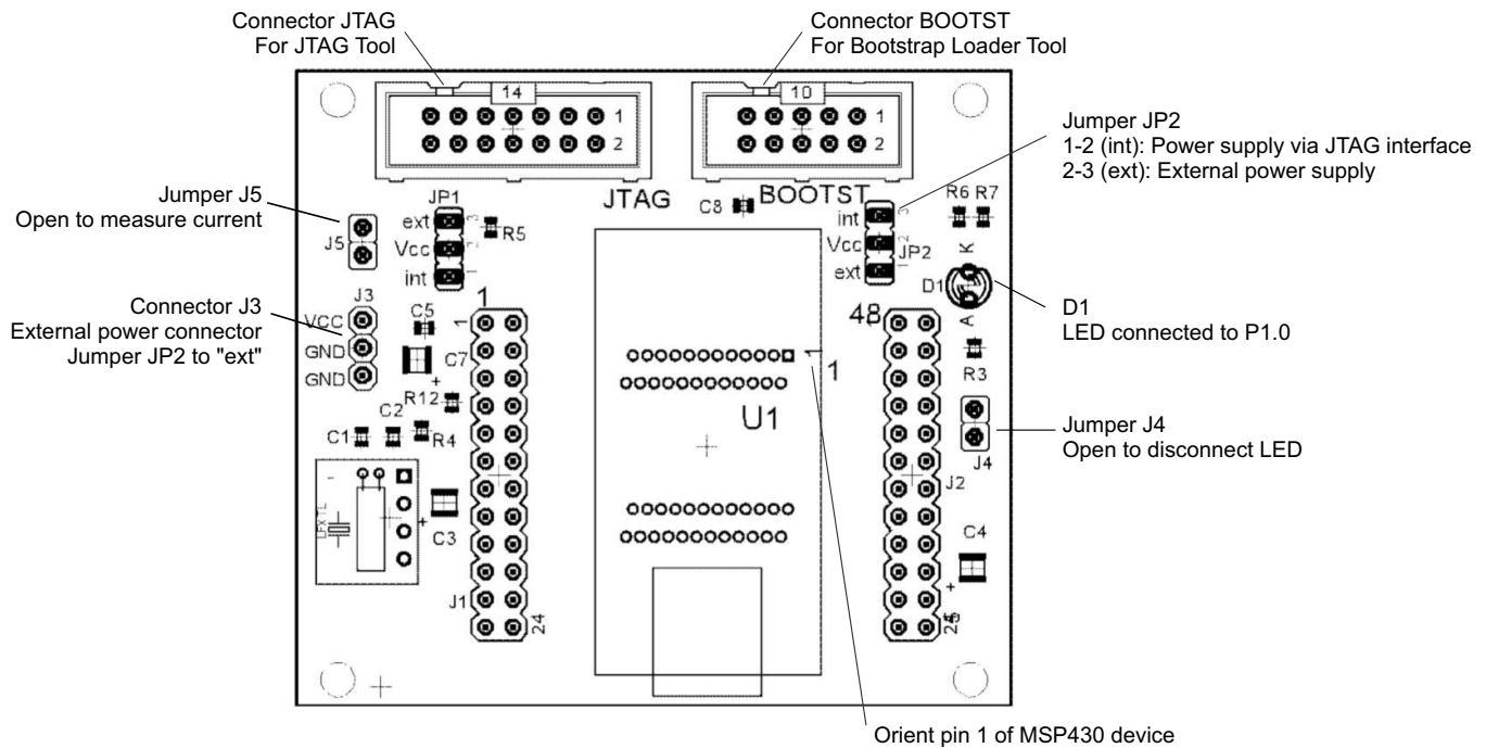
Figure B-28. MSP-TS430DL48 Target Socket Module, PCB
