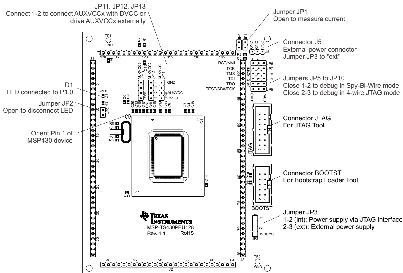
Figure B-68. MSP-TS430PEU128 Target Socket Module, PCB
