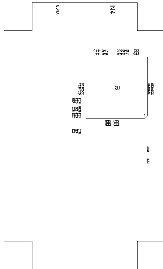
Figure B-83. MSP-FET USB Debugger, PCB (Bottom)
