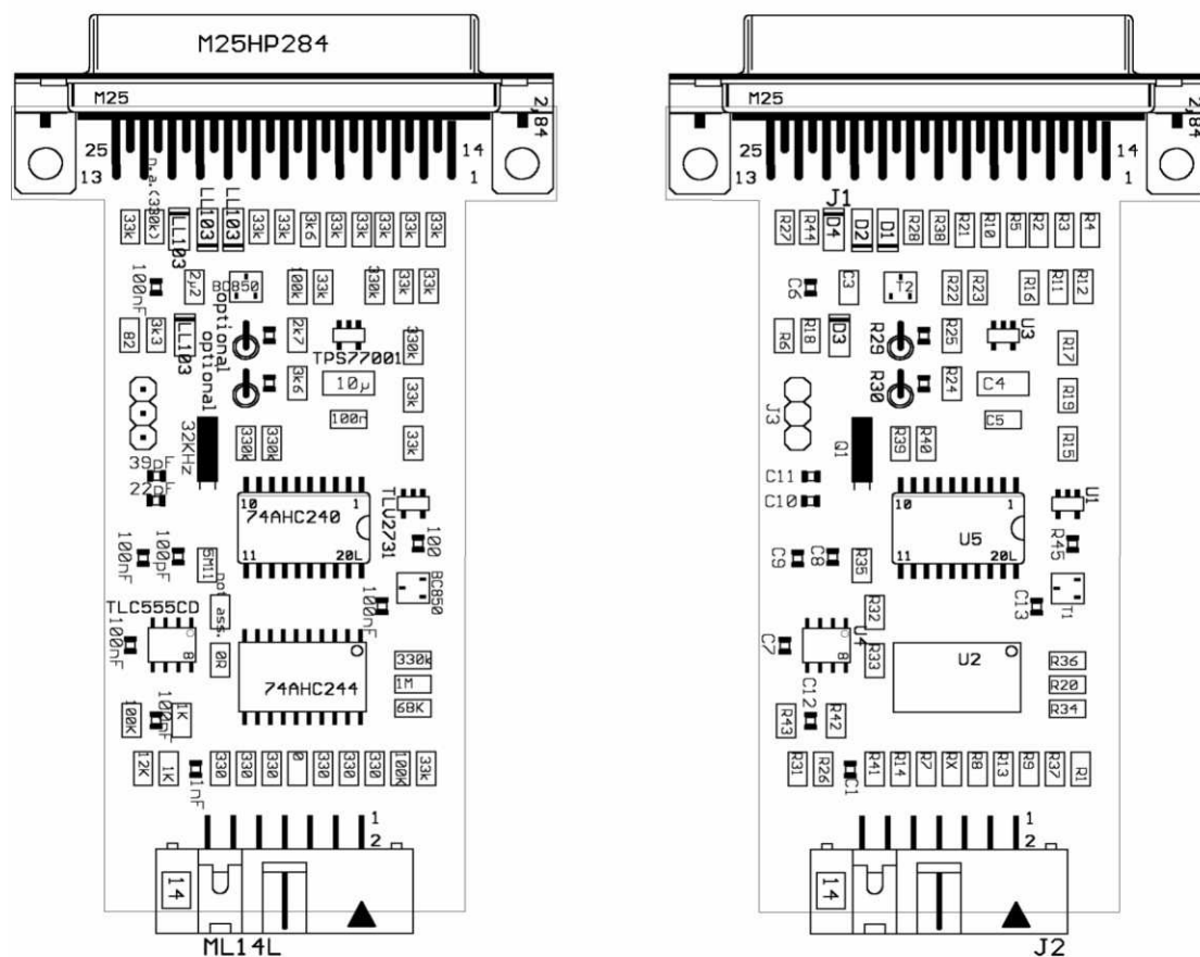
Figure B-87. MSP-FET430PIF FET Interface Module, PCB
