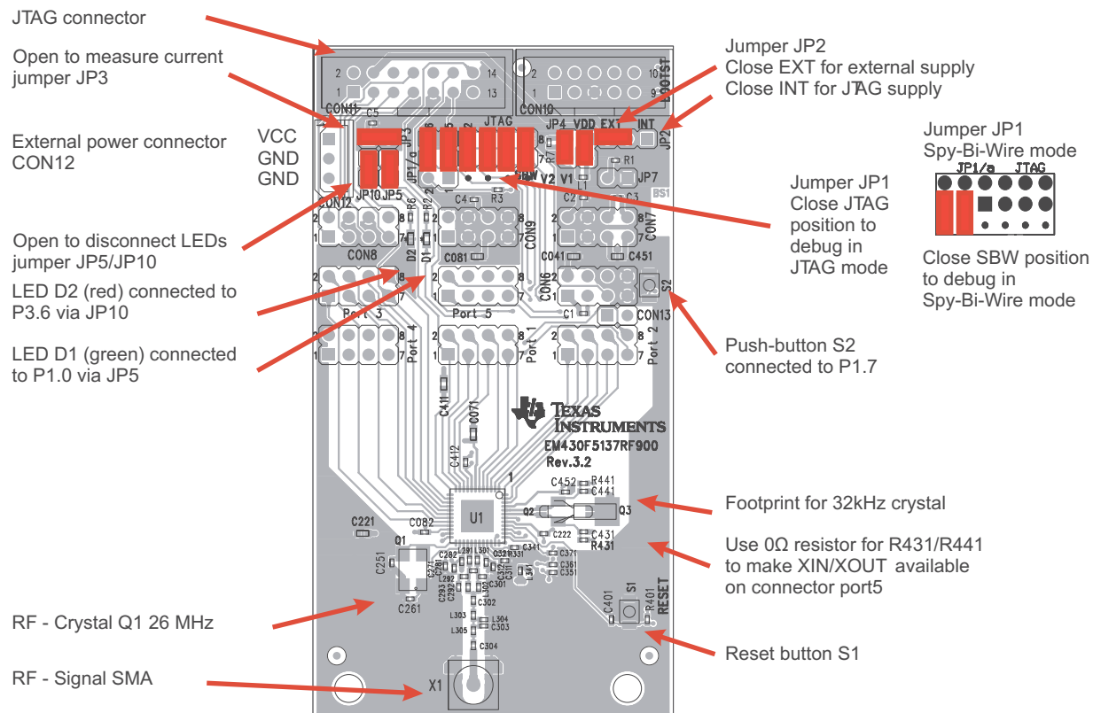
Figure B-70. EM430F5137RF900 Target board, PCB
