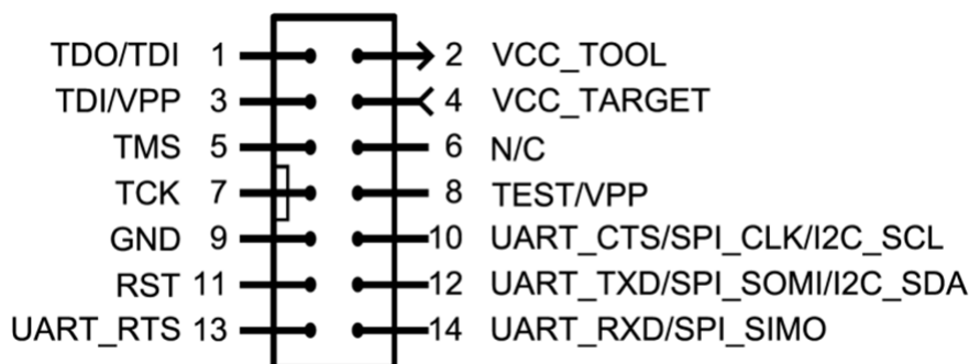
Figure B-84. JTAG Connector Pinout
