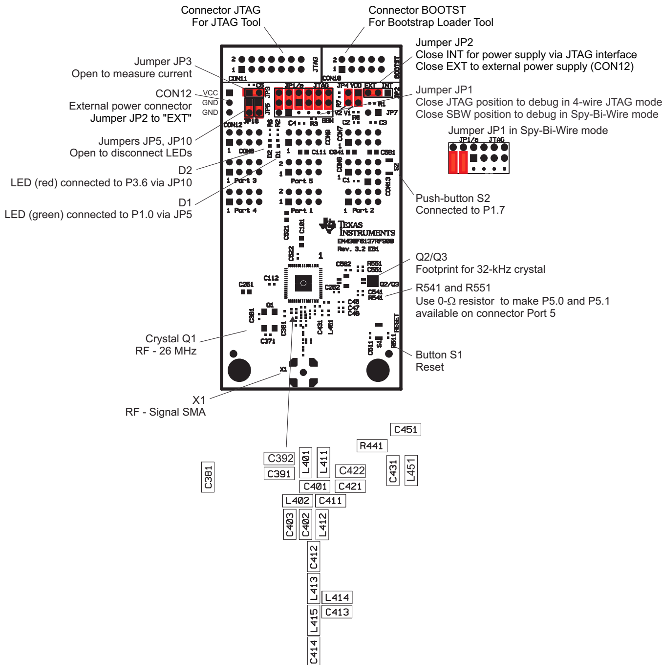
Figure B-72. EM430F6137RF900 Target Board, PCB
