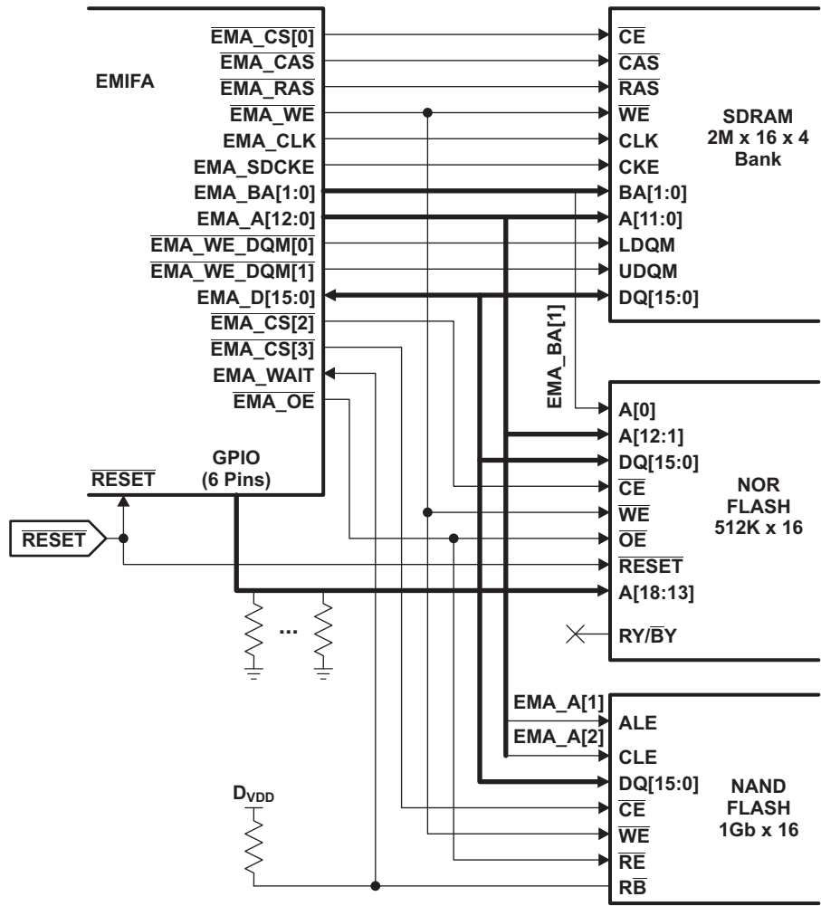
Figure 6-10. OMAP-L138 Connection Diagram: SDRAM, NOR, NAND
