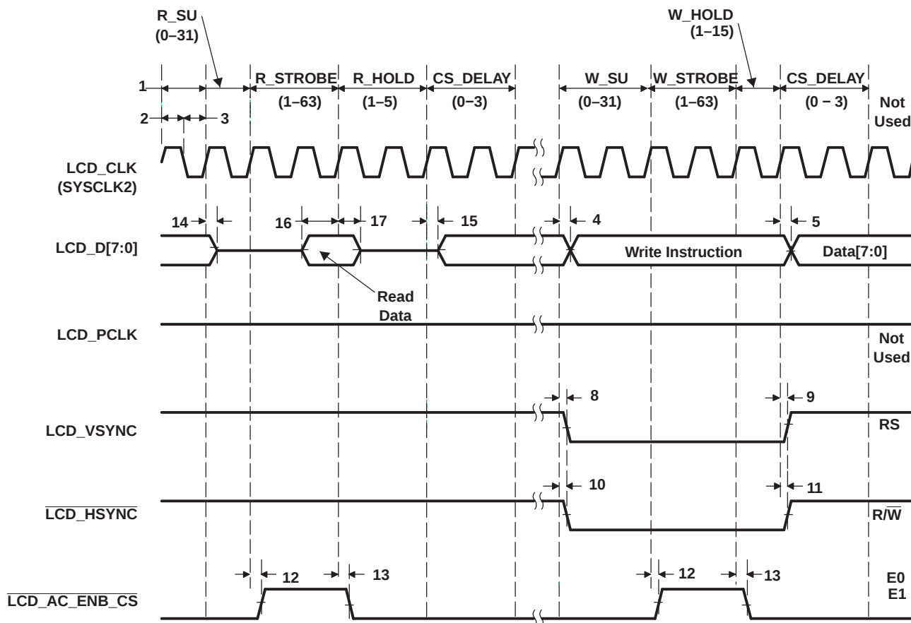
Figure 6-55. Character Display HD44780 Read
