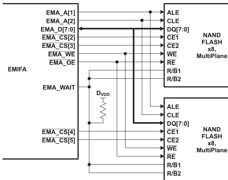
Figure 6-11. OMAP-L138 EMIFA Connection Diagram: Multiple NAND Flash Planes
