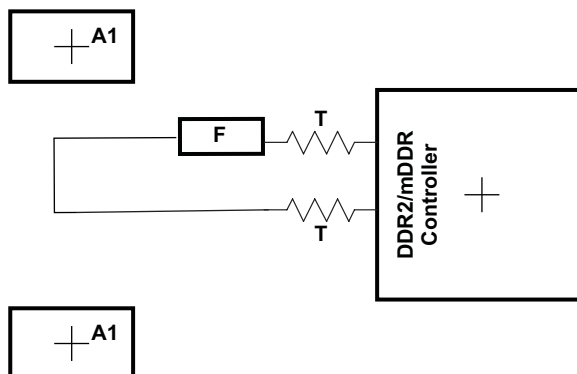
Figure 6-25. DQGATE Routing
