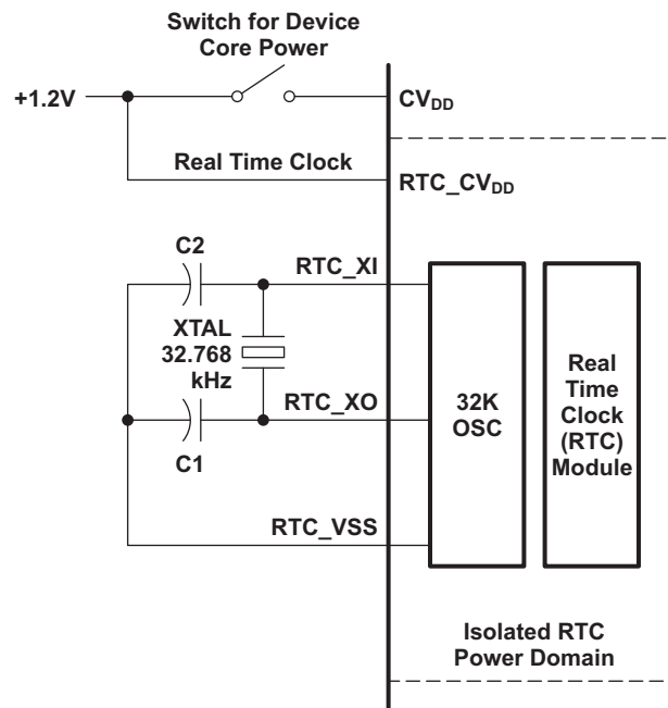
Figure 6-85. Clock Source
