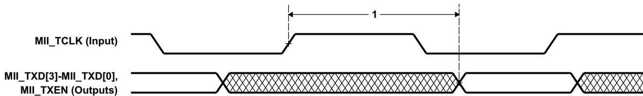
Figure 6-50. EMAC Transmit Interface Timing
