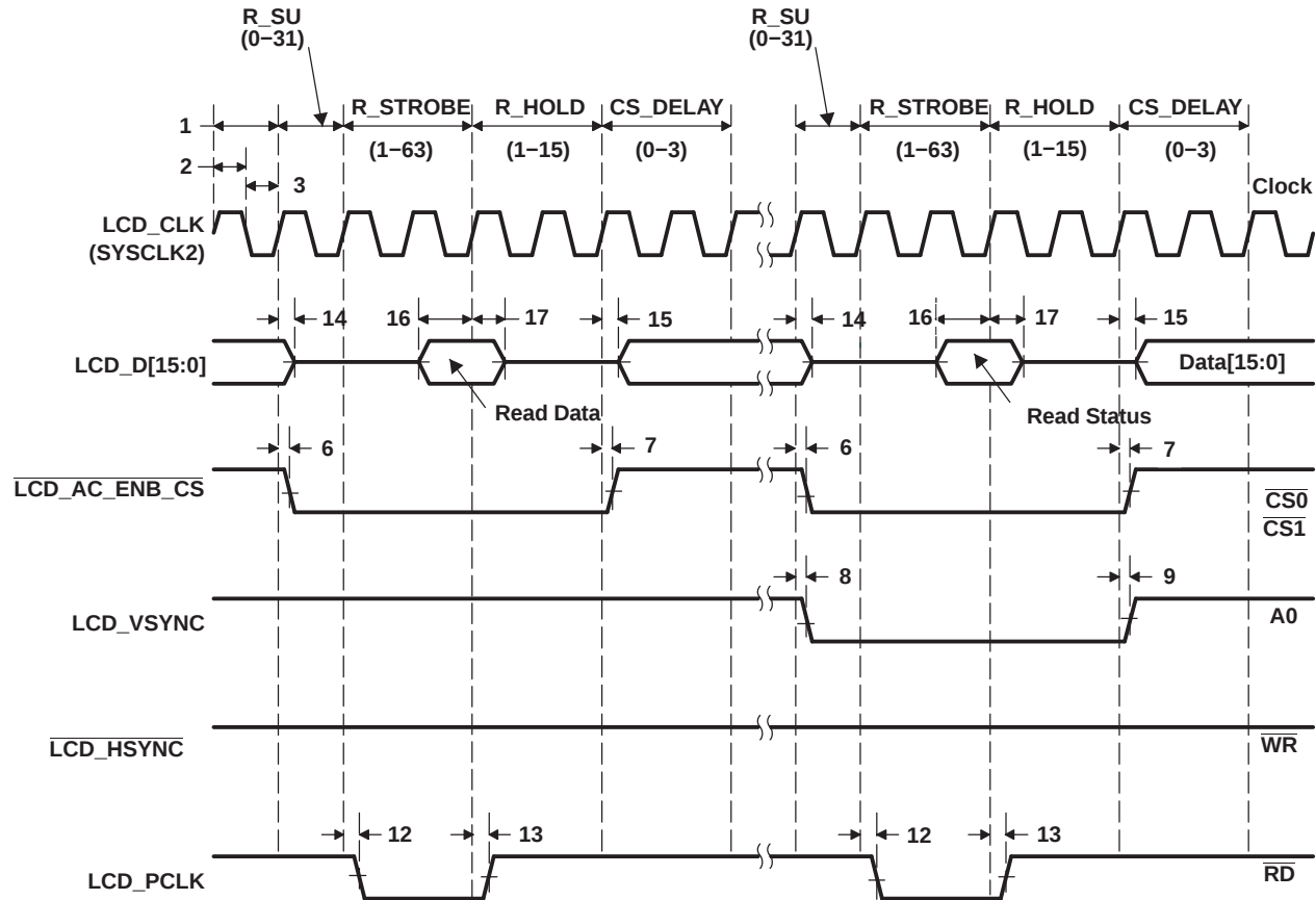
Figure 6-60. Micro-Interface Graphic Display 8080 Status
