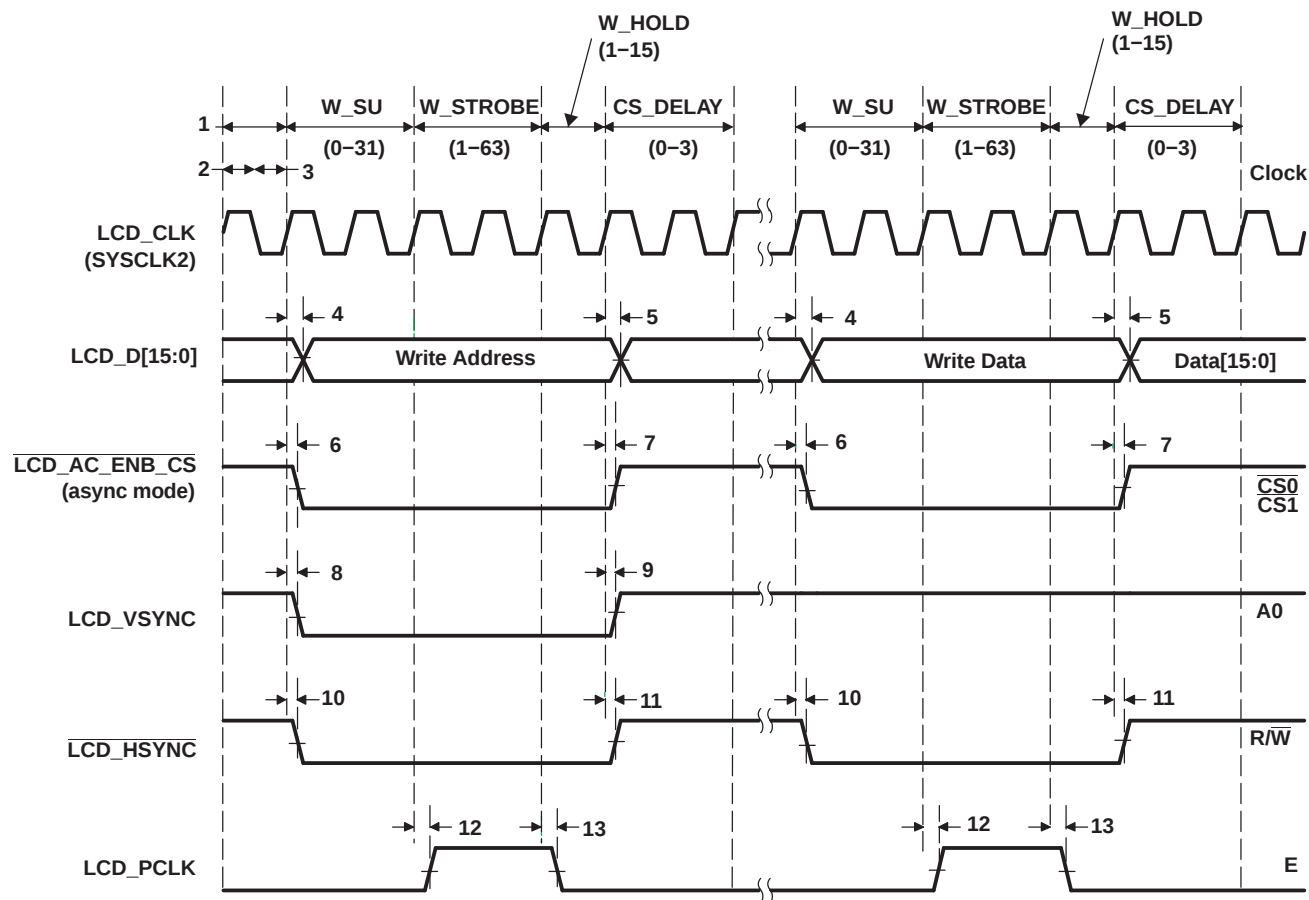
Figure 6-55. Micro-Interface Graphic Display 6800 Write
