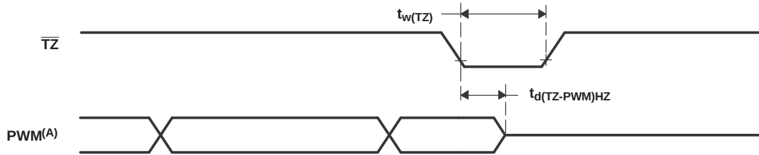
Figure 6-80. PWM Hi-Z Characteristics
