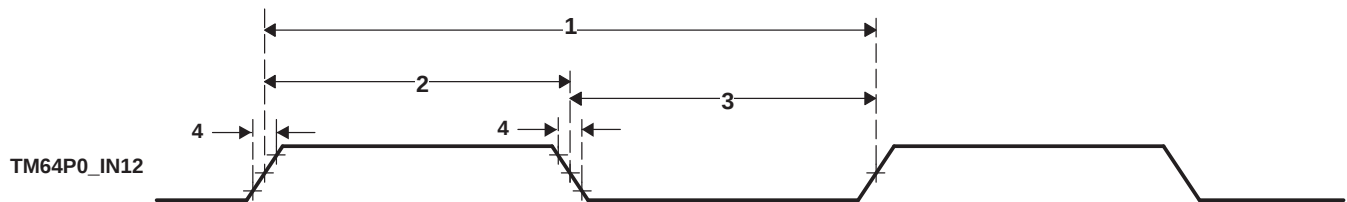
Figure 6-81. Timer Timing
