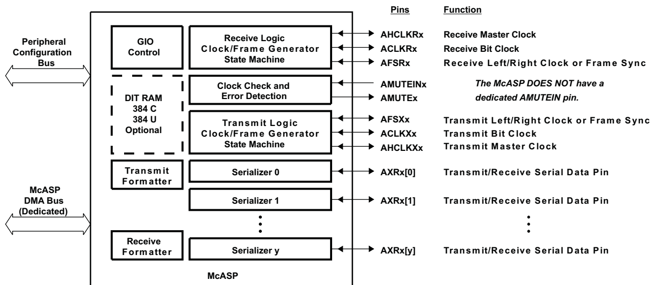
Figure 6-30. McASP Block Diagram
