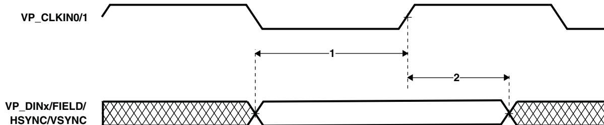
Figure 6-75. VPIF Channels 0/1 Video Capture Data and Control Input Timing
