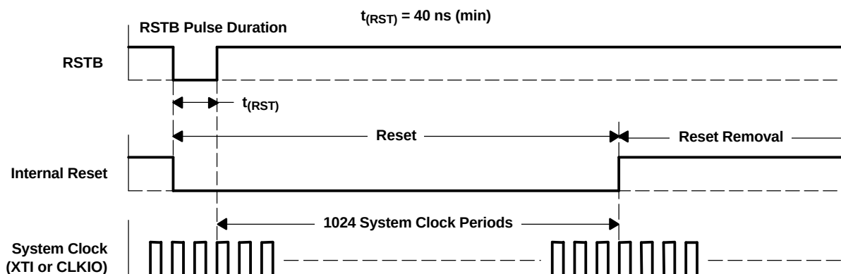
Figure 27. External Forced-Reset Timing
