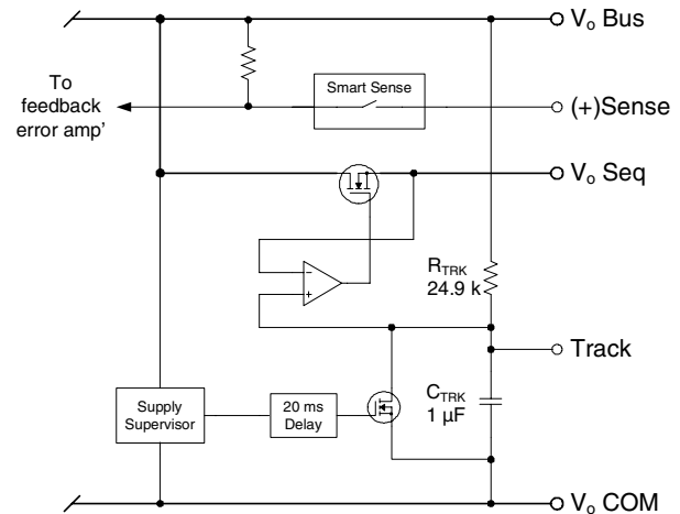
Figure 2-1; Block Diagram of PTB78520W Auto-Track Features
