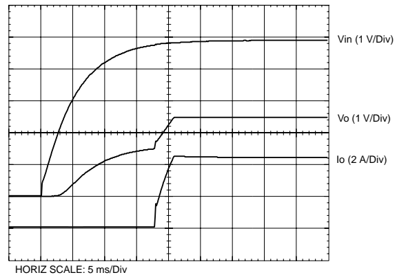
Figure 3-2; Start-up with Output Pre-Bias
