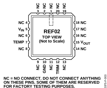
Figure 3. 20-Terminal LCC (RC-Suffix)
