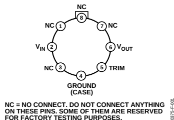
Figure 1. 8-Lead TO-99 (J-Suffix)
