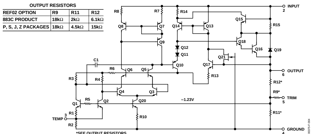
Figure 4. Simplified Schematic
