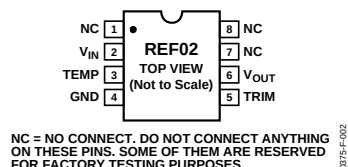
Figure 2. 8-Lead PDIP (P-Suffix), 8-Lead Cerdip (Z-Suffix) and 8-Lead SOIC (S-Suffix)
