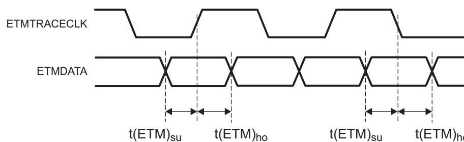
Figure 7-20. ETMDATA Timing
