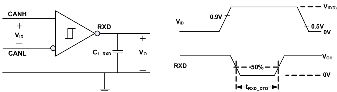
Figure 7. RXD Dominant Timeout Test Circuit and Measurement
