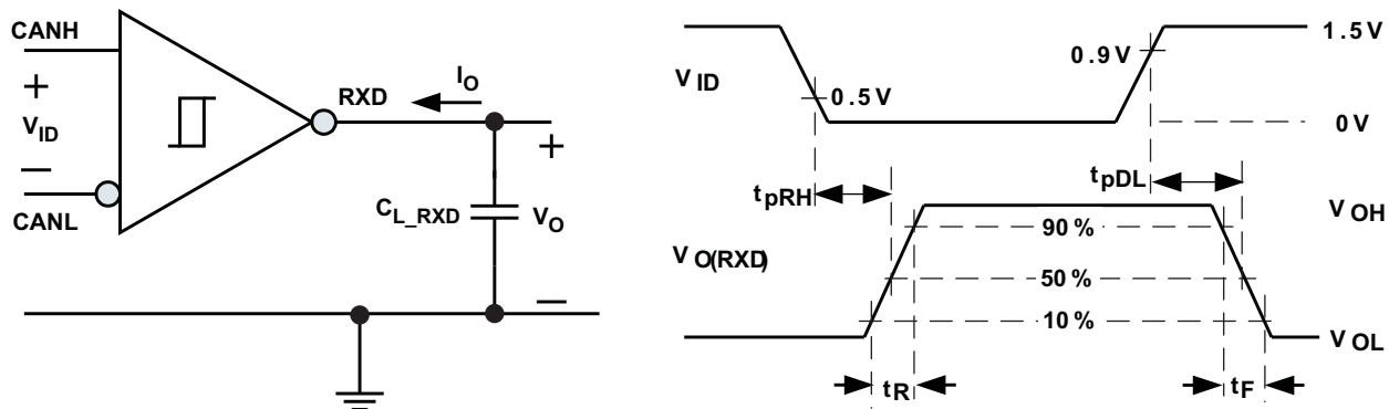
Figure 10. Receiver Test Circuit and Measurement
