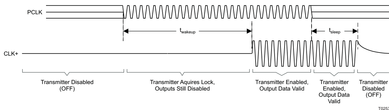
Figure 14. Standby Detection
