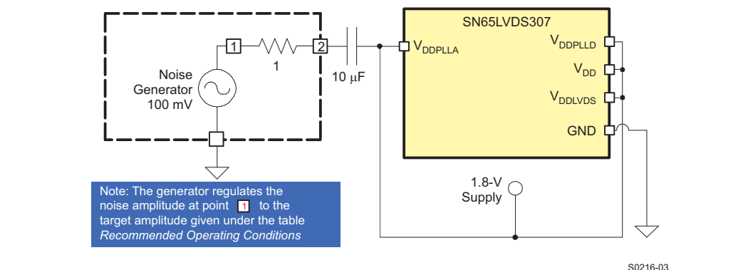
Figure 10. Power Supply Noise Test Setup
