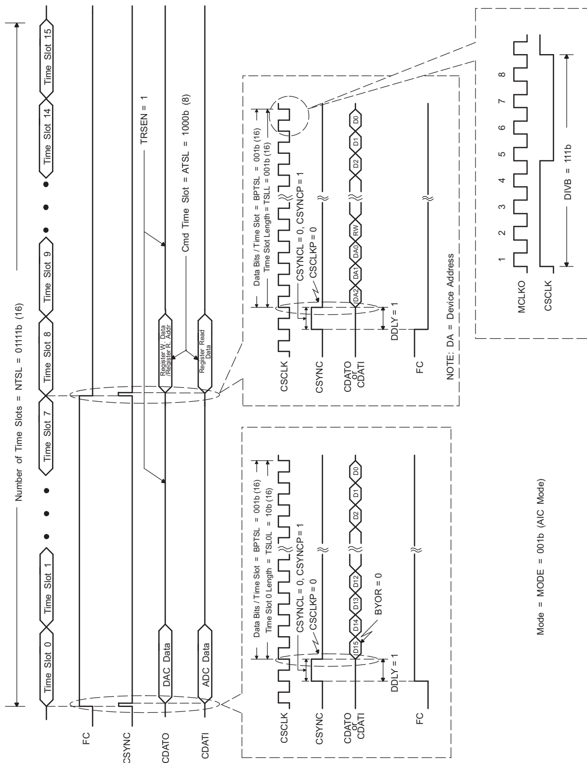
Figure 2-7. Codec Port Interface Parameters – AIC
