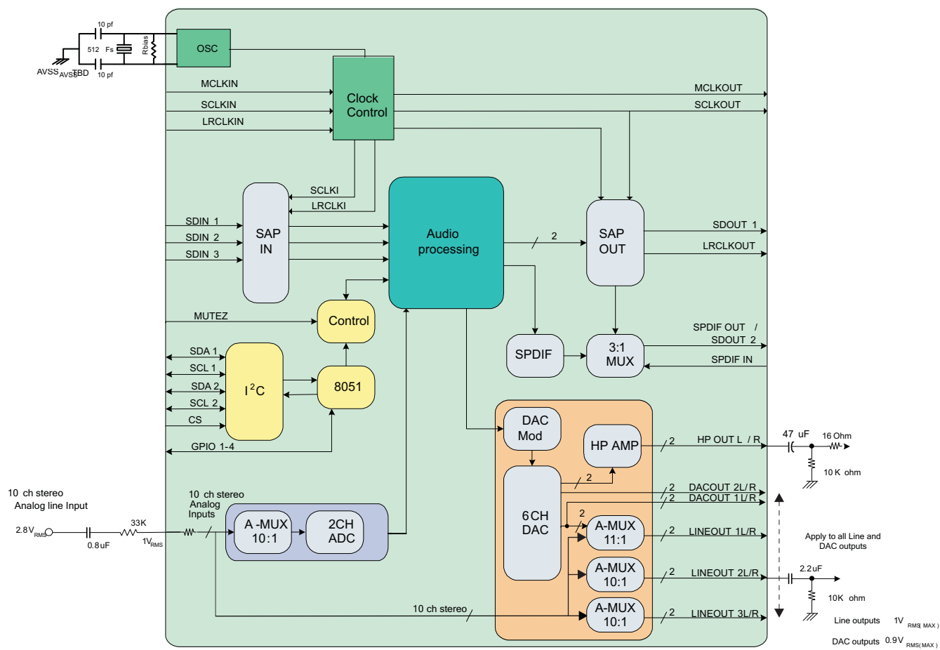
Figure 1. Block Diagram
