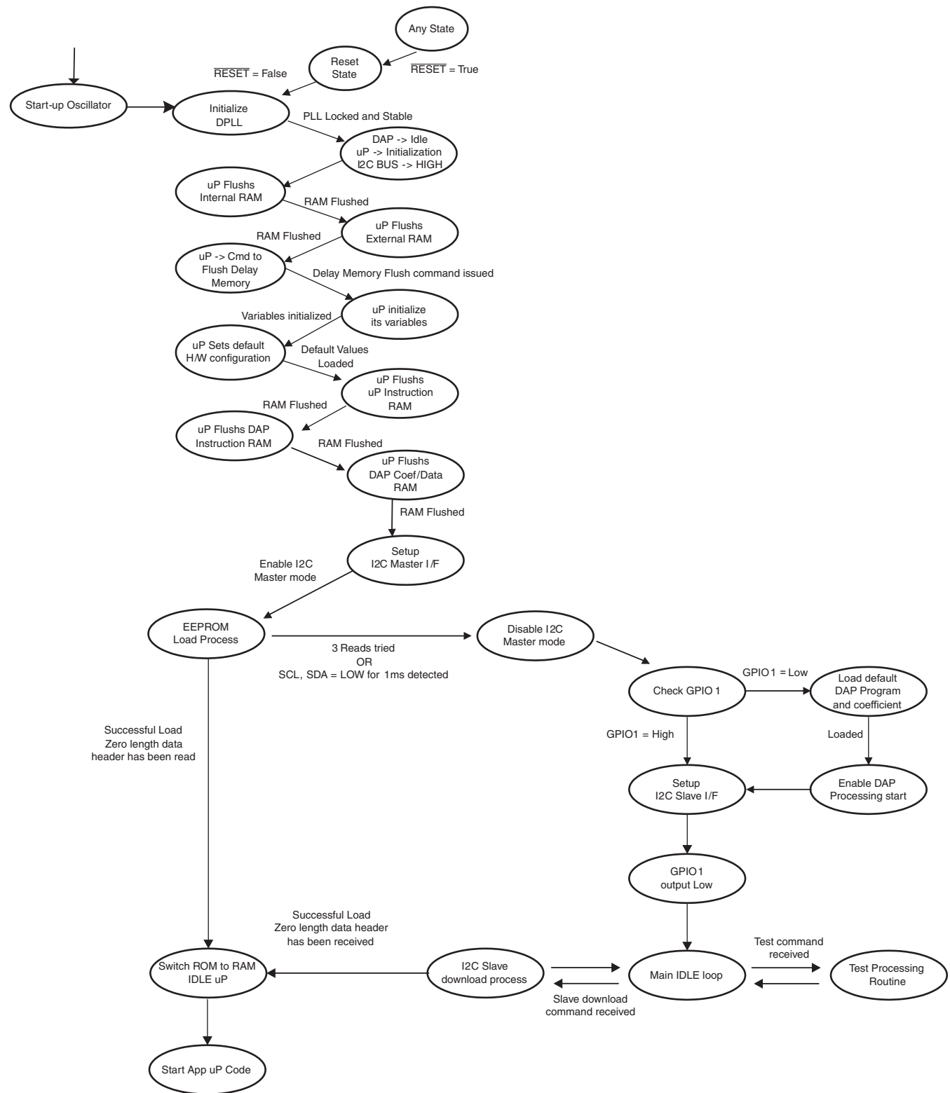
Figure 17. Boot-Up Sequence
