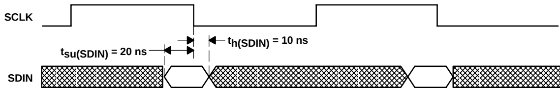
Figure 4-5. DSP Serial Port Expanded Timing
