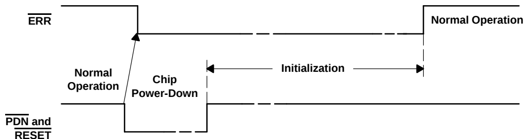
Figure 2-4. Power-Down Timing
