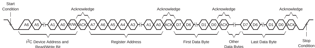
Figure 2-15. Multiple-Byte Write Transfer
