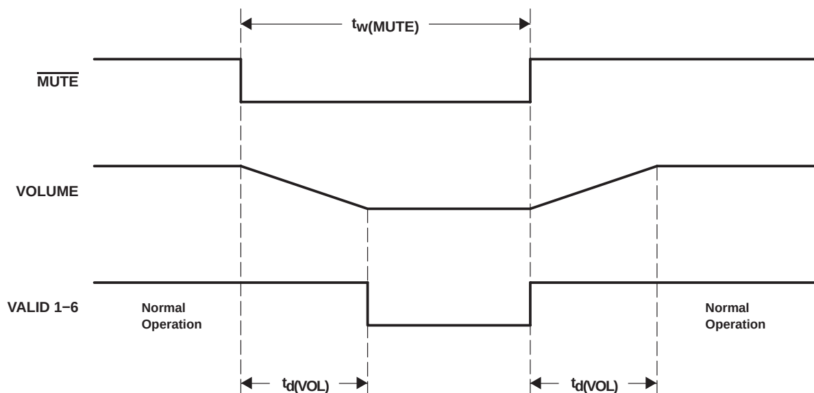
Figure 5-5. Mute Timing
