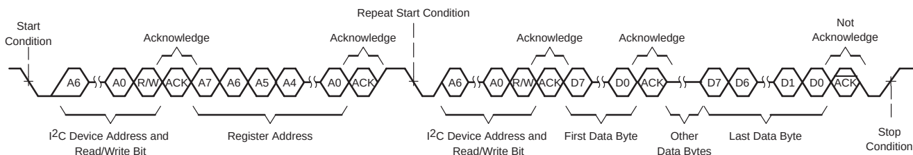
Figure 2-17. Multiple-Byte Read
