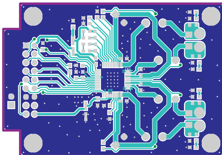
Figure 20. TAS5709EVM (TAS5707EVM) Top Copper Assembly
