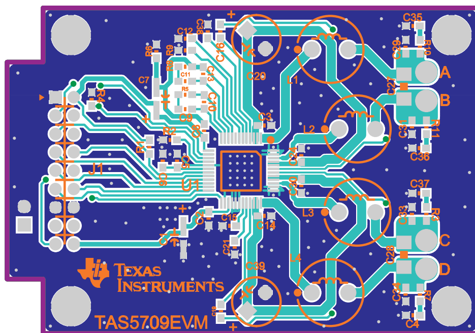
Figure 19. TAS5709EVM(TAS5707EVM) Top Composite Assembly
