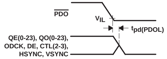
Figure 8. Delay From \overline{\text{PDL}} Low to Hi-Z Outputs
