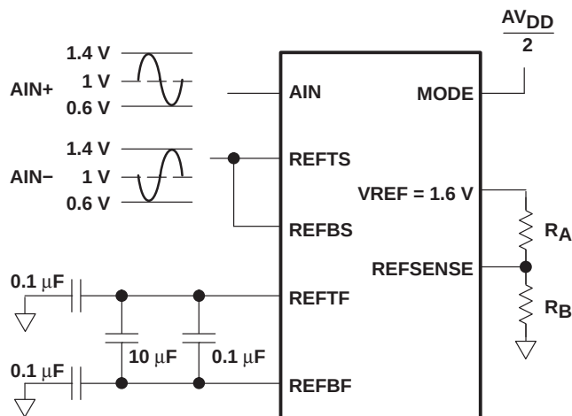
Figure 25. Differential Operation
