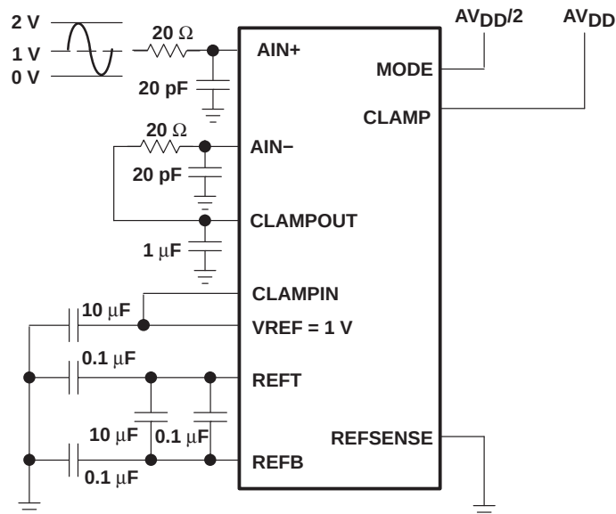
Figure 34. Operating Configuration: 2-V Single-Ended Input, Internal ADC References
