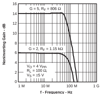
NONINVERTING LARGE SIGNAL FREQUENCY RESPONSE
