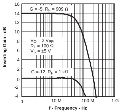
INVERTING LARGE SIGNAL FREQUENCY RESPONSE
