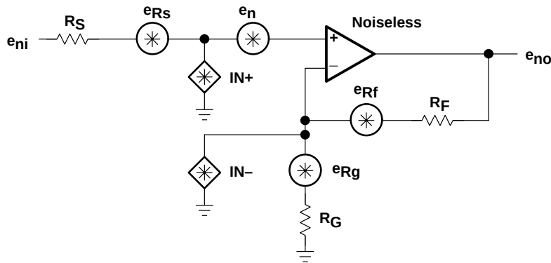
Figure 41. Noise Model
