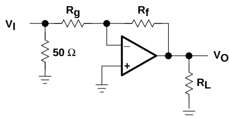
Figure 4. Step Response Test Circuit
