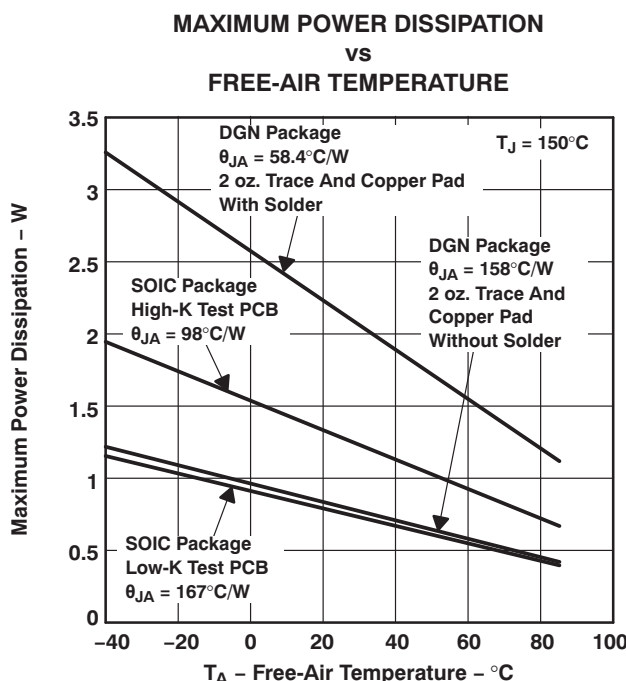
Figure 49. Maximum Power Dissipation vs Free-Air Temperature
