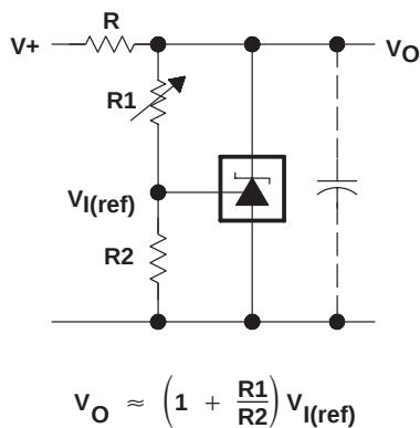
Figure 5. Shunt Regulator
