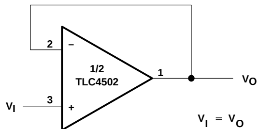
Figure 40. Voltage-Follower Circuit
