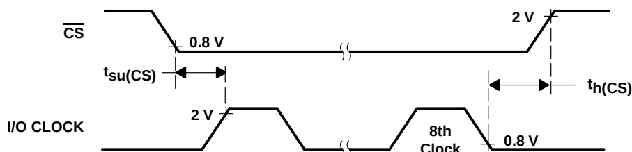
Figure 4. \overline{\text{CS}} to I/O CLOCK Timing
