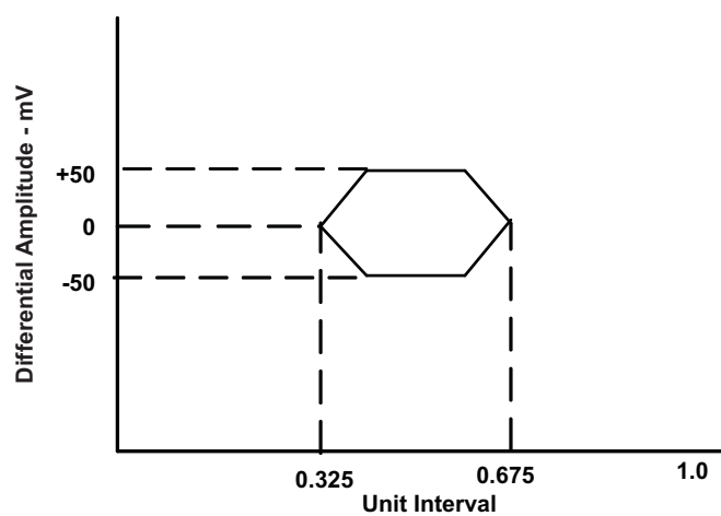
Figure 34. Receive Template
