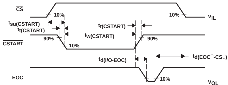
Figure 15. CSTART and CS Waveforms
