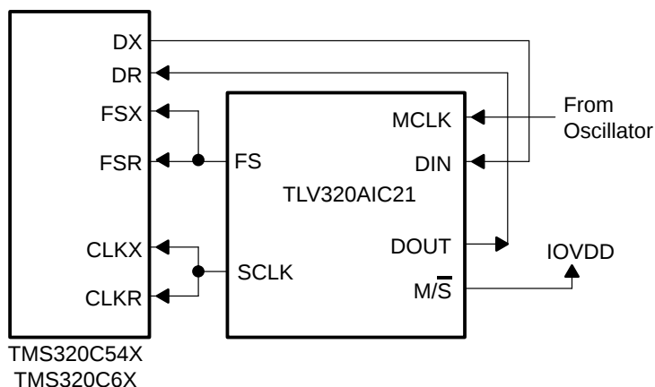
Figure 5–19. TLV320AIC21s Interface to McBSP Port of C54x or C6x DSP
