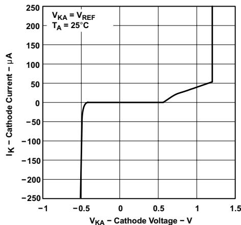
Figure 8. Cathode Current vs Cathode Voltage
