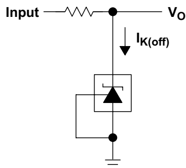
Figure 3. Test Circuit for I_{K(off)}
