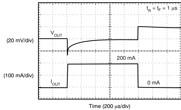
LOAD TRANSIENT 0
