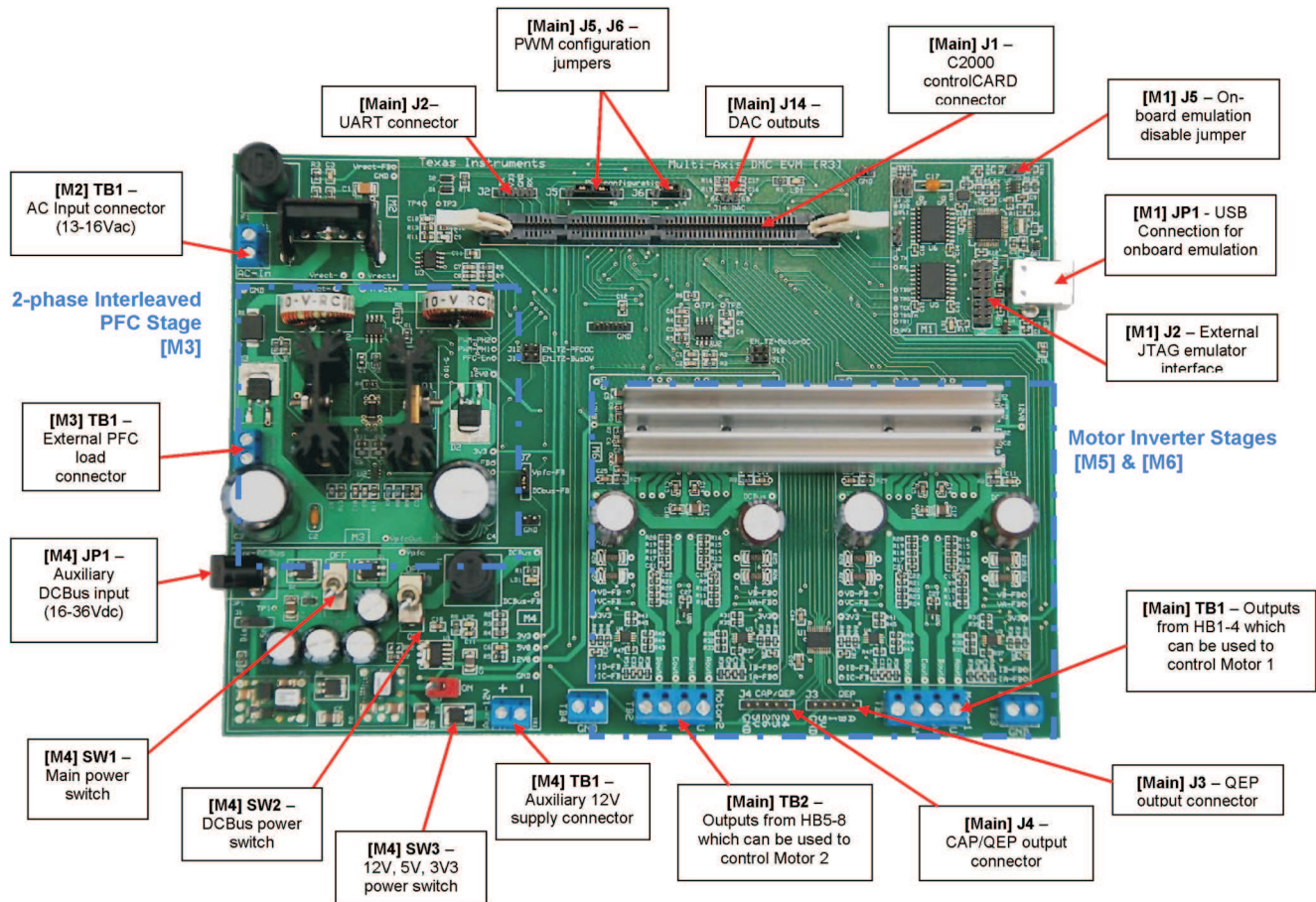
Figure 1. Hardware Overview
