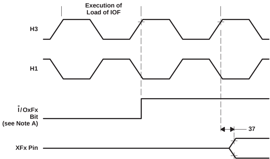
Figure 20. Timing for Change of XFx From Input to Output Mode
