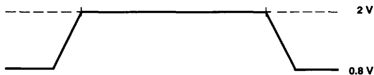
Figure 6. TTL-Level Inputs
