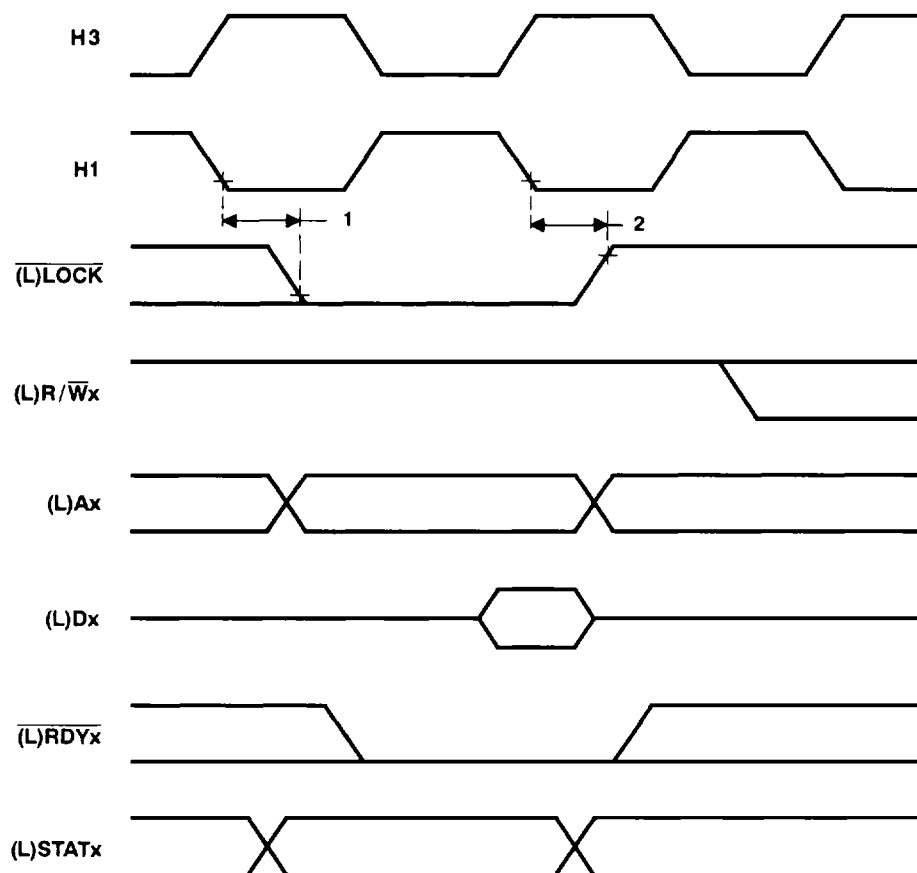
Figure 14. Timing for \overline{(L)}\text{LOCK} When Executing SIGI
