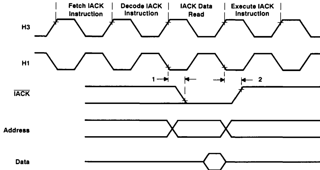
Figure 21. \overline{\text{IACK}} Timing
