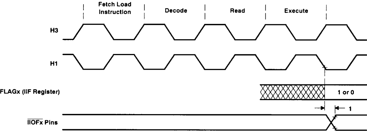
Figure 16. Timing for the \overline{\text{IIOF}}_x When Configured as an Output
