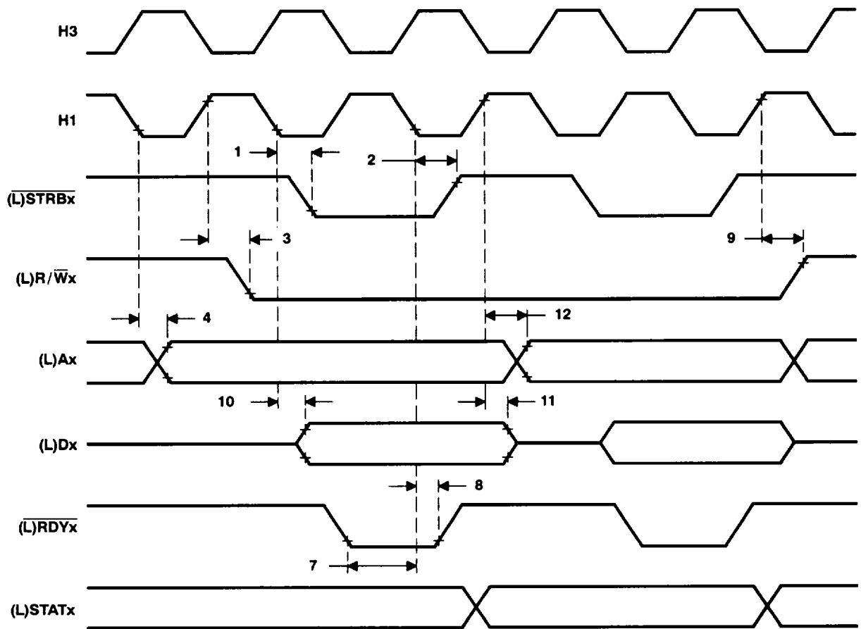
Figure 10. Memory-Write-Cycle Timing [(L)STRBx = 0]
