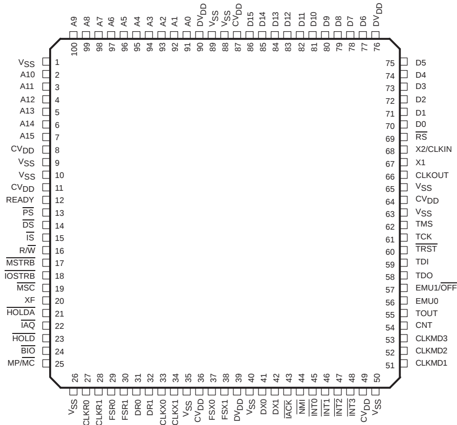
TMS320C541, TMS320LC541 PZ PACKAGE† (TOP VIEW)
