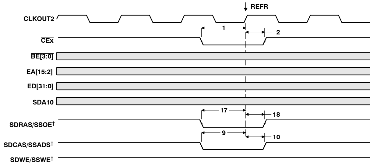
Figure 29. SDRAM REFRESH Command
