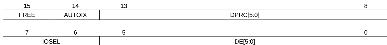
Figure 3-19. DMPREC Register
