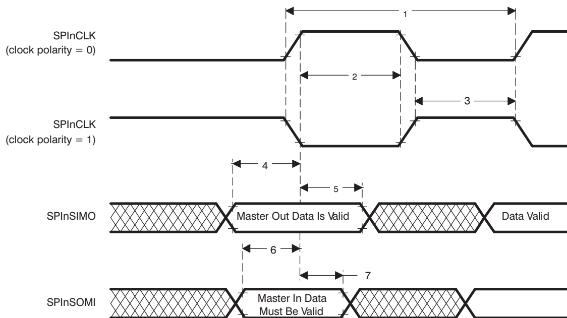
Figure 14. SPI Master Mode External Timing (CLOCK PHASE = 1)
