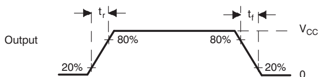
Figure 11. CMOS-Level Outputs
