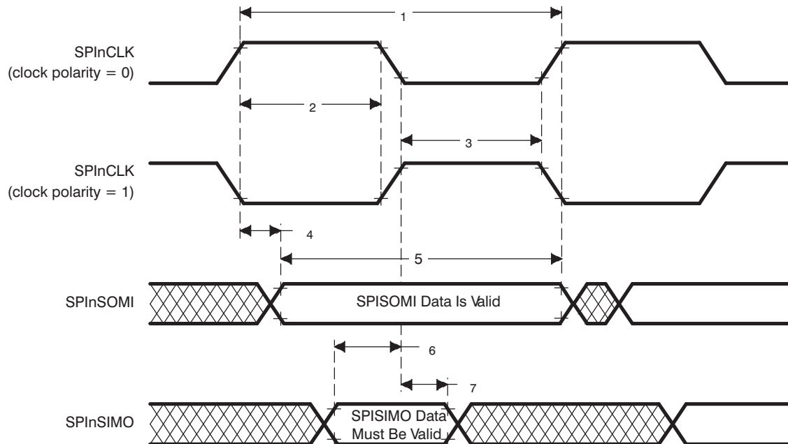
Figure 15. SPI IN Slave Mode External Timing (CLOCK PHASE = 0)
