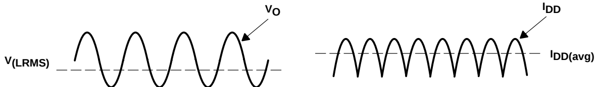
Figure 35. Voltage and Current Waveforms for BTL Amplifiers
