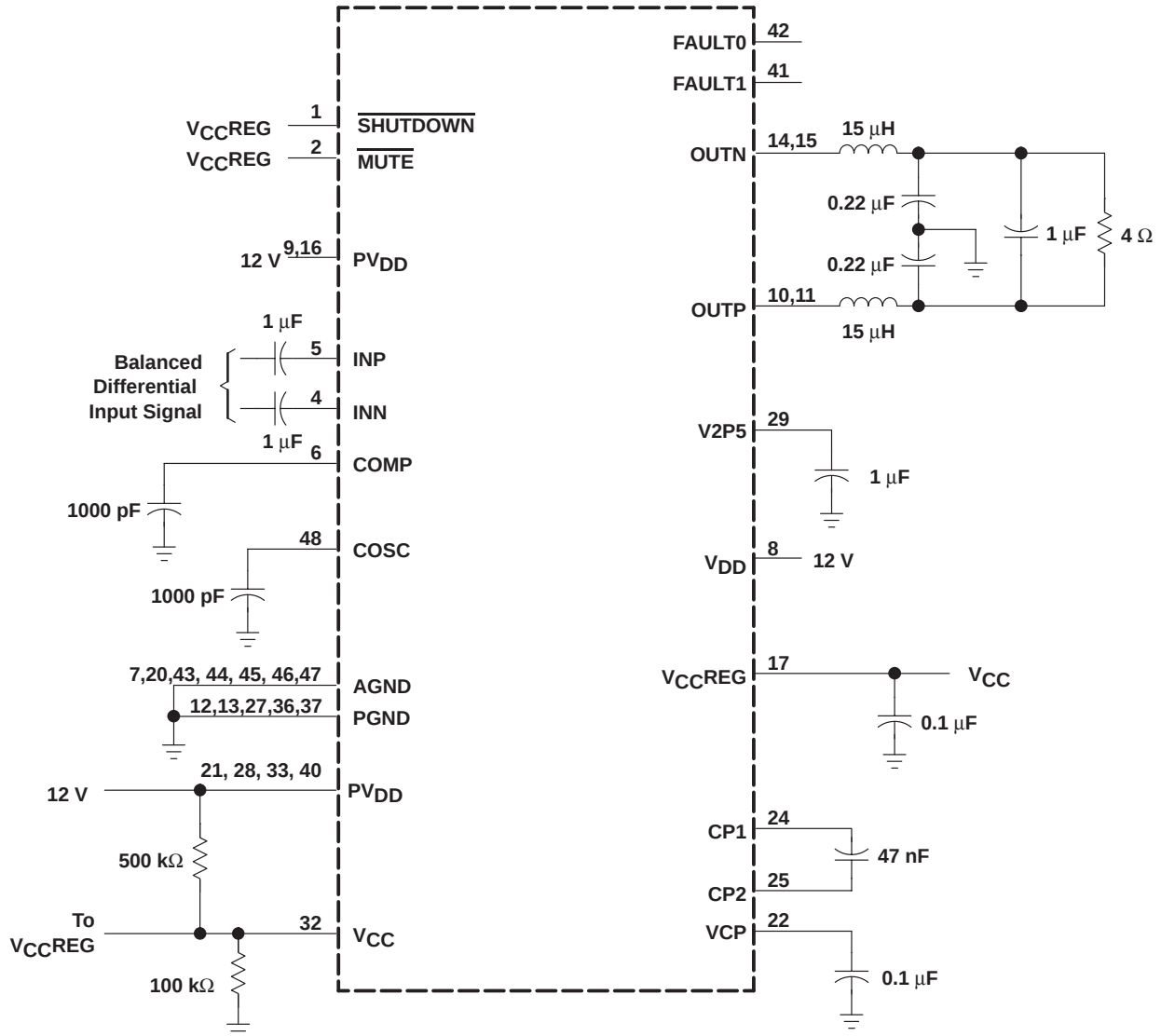
Figure 1. 12-V, 4- \Omega Test Circuit
