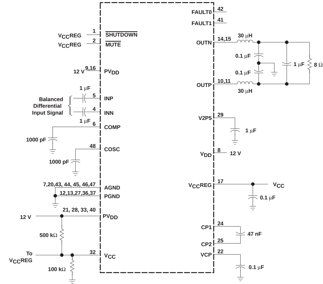
Figure 2. 12-V, 8- \Omega Test Circuit
