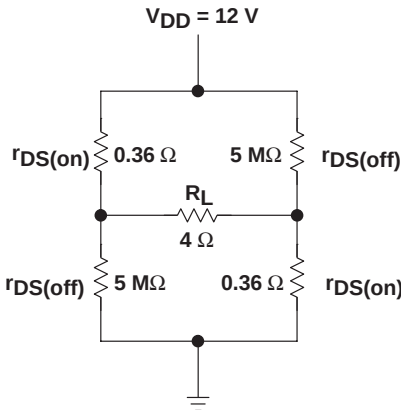
Figure 8. Output Transistor Simplification for Conduction Loss Calculation
