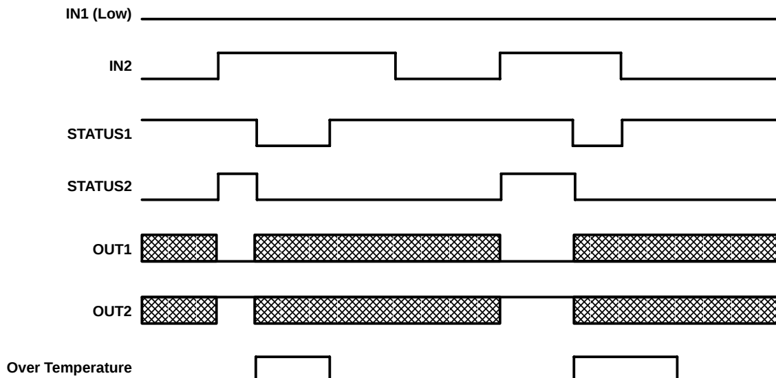
Figure 4. Over Temperature
