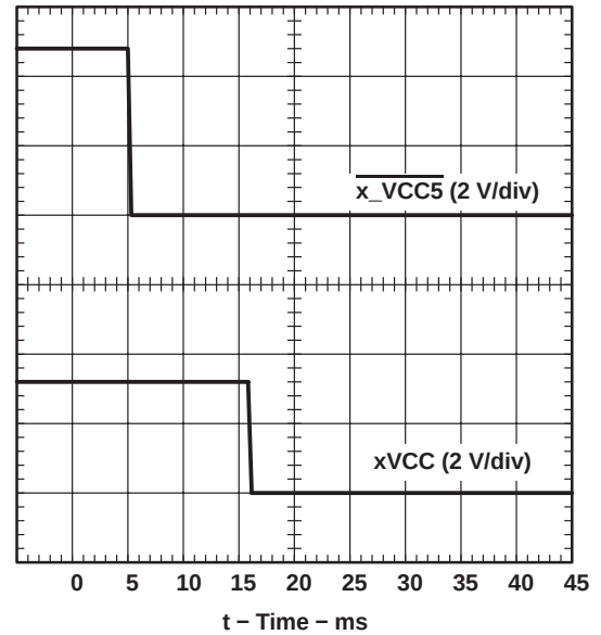
Figure 3. xVCC Propagation Delay and Fall Time With 1-μF Load, 3.3-V Switch, ( V_{I(5V)} = 5 V)
