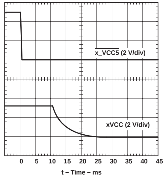
Figure 5. xVCC Propagation Delay and Fall Time With 150-μF Load, 3.3-V Switch, V_{I(5V)} = 5 V
