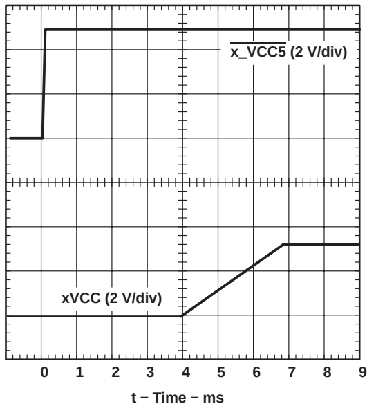
Figure 4. xVCC Propagation Delay and Rise Time With 150-μF Load, 3.3-V Switch, V_{I(5V)} = 5 V
