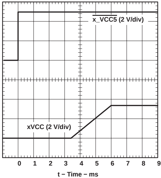
Figure 2. xVCC Propagation Delay and Rise Time With 1-μF Load, 3.3-V Switch, ( V_{I(5V)} = 5 V)
