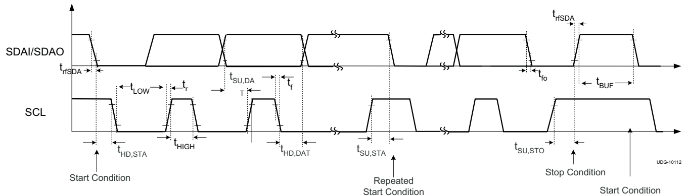
Figure 24. I²C Timings
