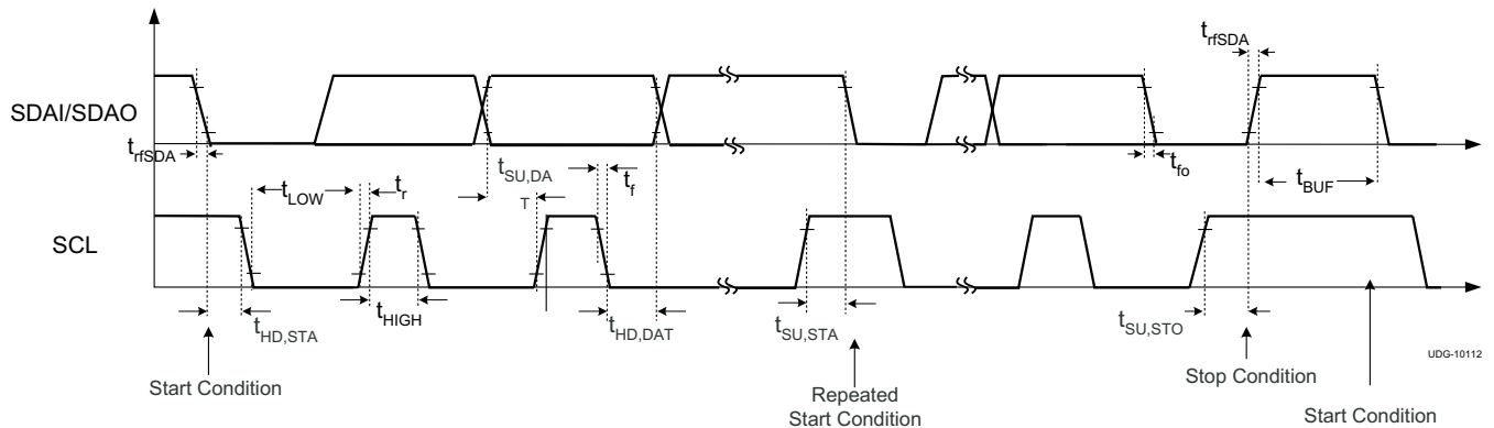
Figure 25. I²C Timings
