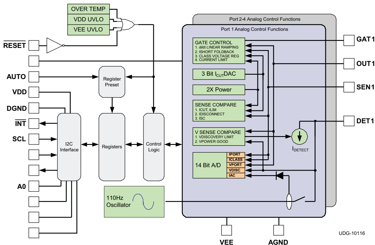
Figure 24. Block Diagram
