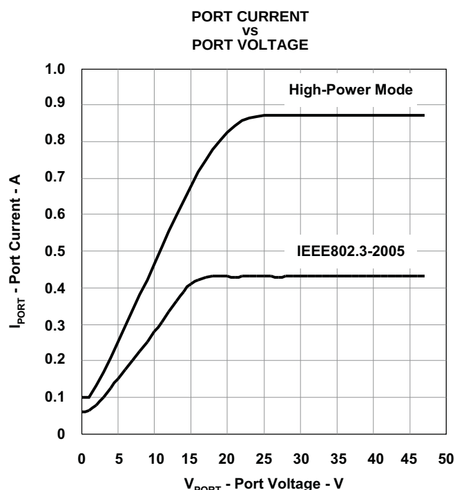
Figure 29. Output Current Foldback Function (In IEEE Std 802.3at-2009 Mode and High-Power Mode)
