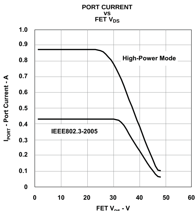
Figure 30. Output Current Foldback Function (With VEE = -48 V, in IEEE Std 802.3at-2009 Mode and High-Power Mode)
