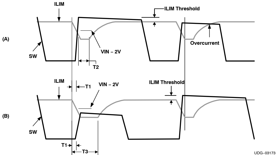
Figure 10. Switching and Current Limit Waveforms and Timing Relationship
